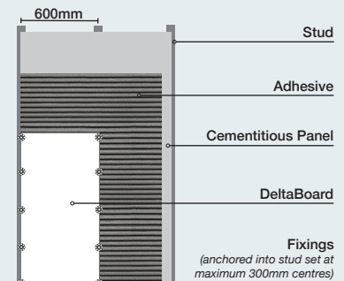
Indicative Fixing Detail using adhesive, washers & screws based on 600mm stud centres (1200mm x 600mm x 20mm DeltaBoard)
